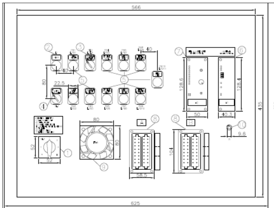
Picture 2. Emergency Console Top View Layout
